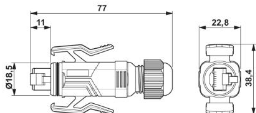
RJ45 plug connector, IP67
